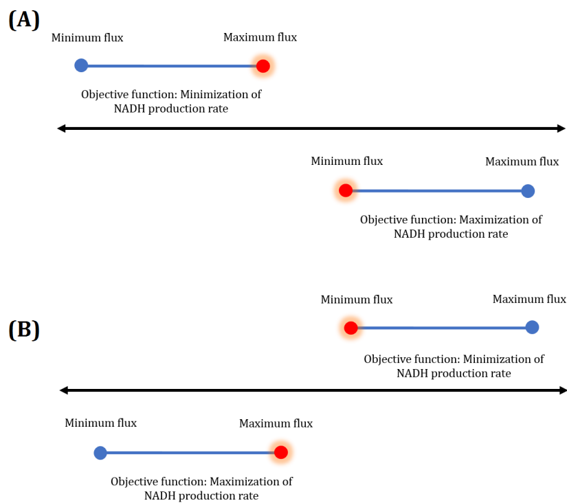
Fig. 1. Comparison of flux variability for each reaction at the minimum and maximum rates of NADH production reaction to finding appropriate reactions for (A) up-regulation, and (B) down-regulation. Compared rates were highlighted in red.
