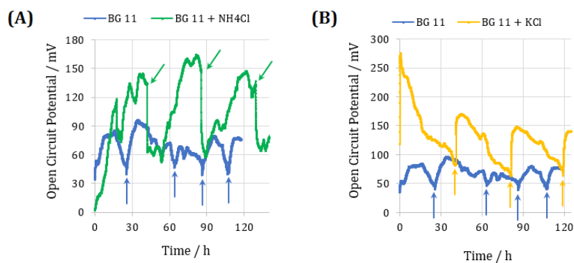
Fig. 4. The open circuit potential (OCP) evolution of three used suspensions for microbial enrichment. (A) Synechocystis + BG-11 and Synechocystis + BG-11 + 40mM NH 4 Cl, (B) Synechocystis + BG-11 and Synechocystis + BG-11 + 50mM KCl.
