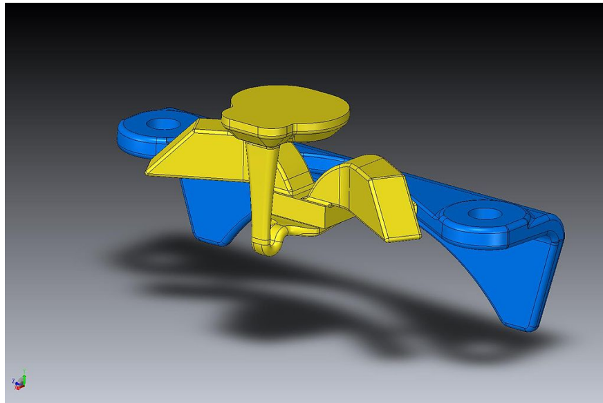
Figure 4: Figure 4: CAD model used for 3D printing.
