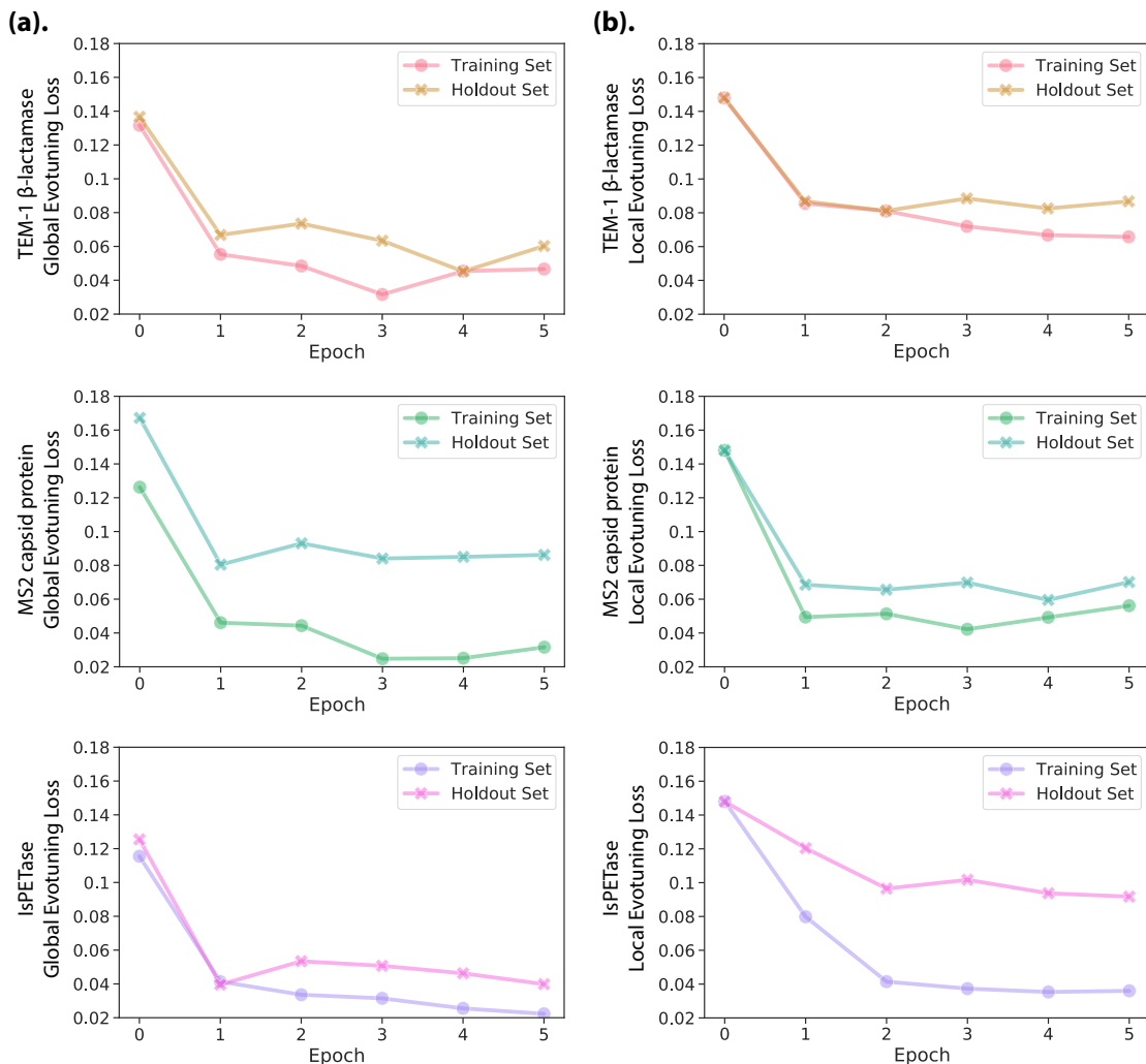
Figure 1: Loss-trajectories for the first five epochs of evotuning procedure for TEM-1 \beta -lactamase, MS2 capsid protein, and IsPETase. (a) . Global evotuning trajectories: parameters are initiated as the globally trained UniRep weights; learning-rate = 10^{-5} . (b) . Local evotuning: parameters are initiated as random values; learning-rate = 10^{-5} .
